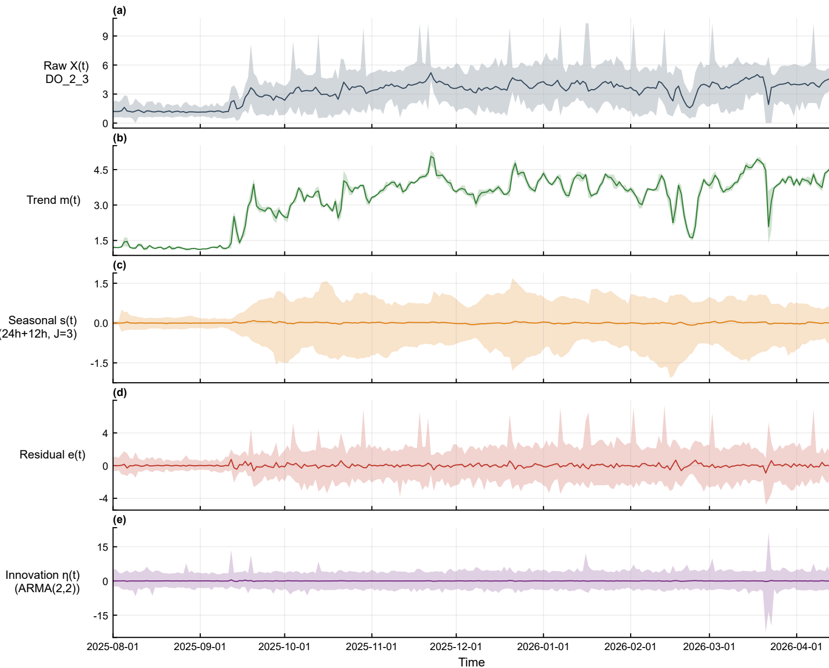
Full-span daily overview — DO_2_3 (aerobic, min) [2025-08-01~2026-04-13]
